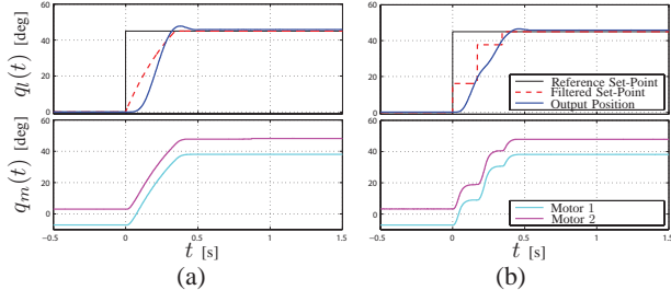
Fig. 7. Response of the system with stiffness preset p^* = 5 to a step input of 45 deg, shaped by exponential jerk filter (a) and ZVD input shaper (b).
