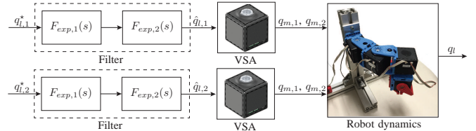
Fig. 9. Block-scheme representation of the feedforward control.
